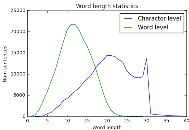
Figure 1: The blue line is character length statistic, and green line is word length .
